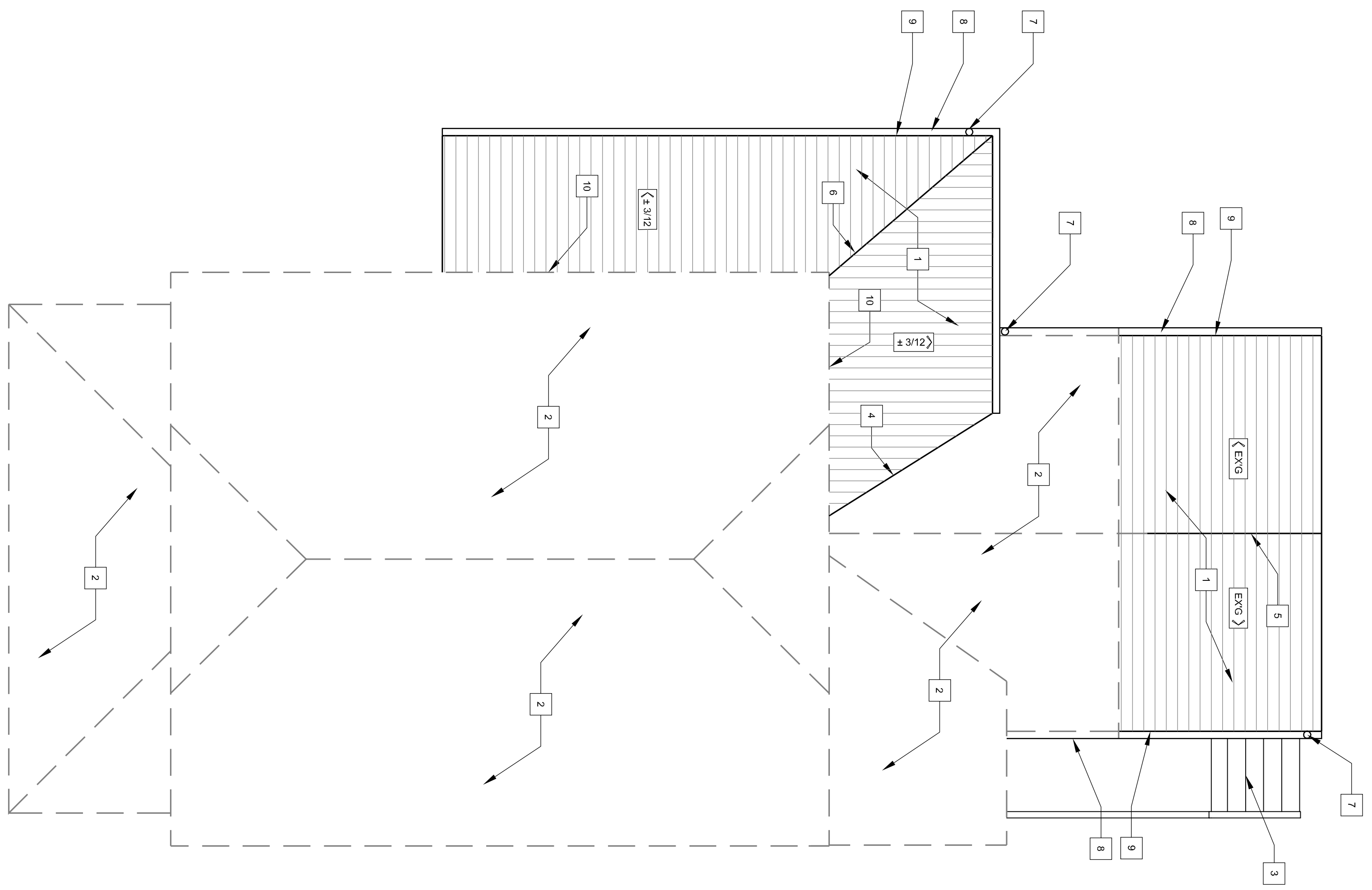
1 ROOF PLAN 1/4" = 1'-0"
