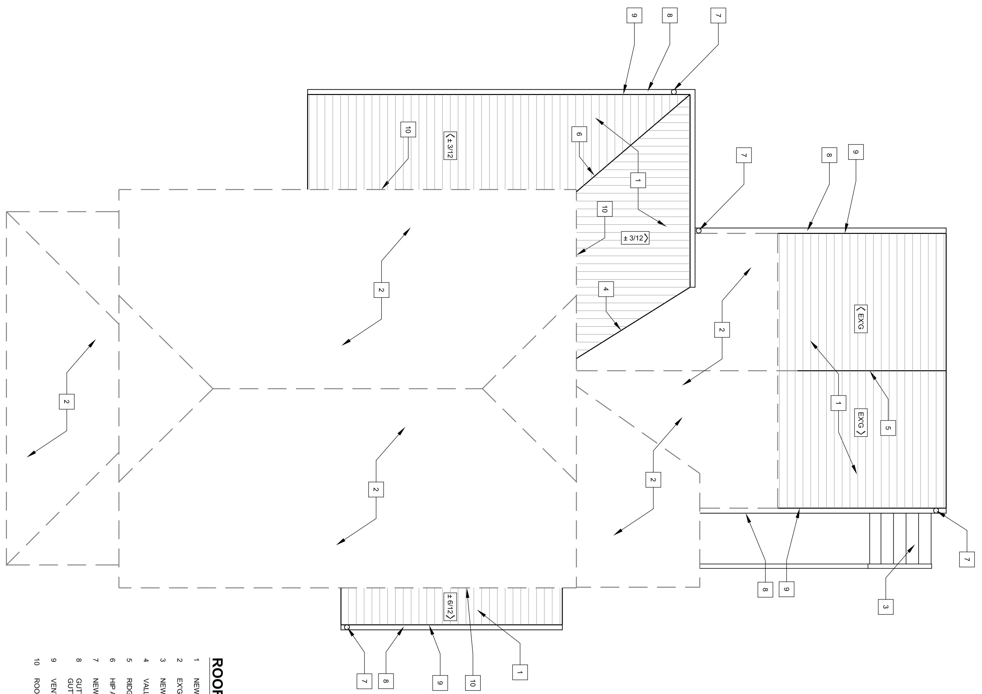
1 ROOF PLAN 1/4" = 1'-0"
