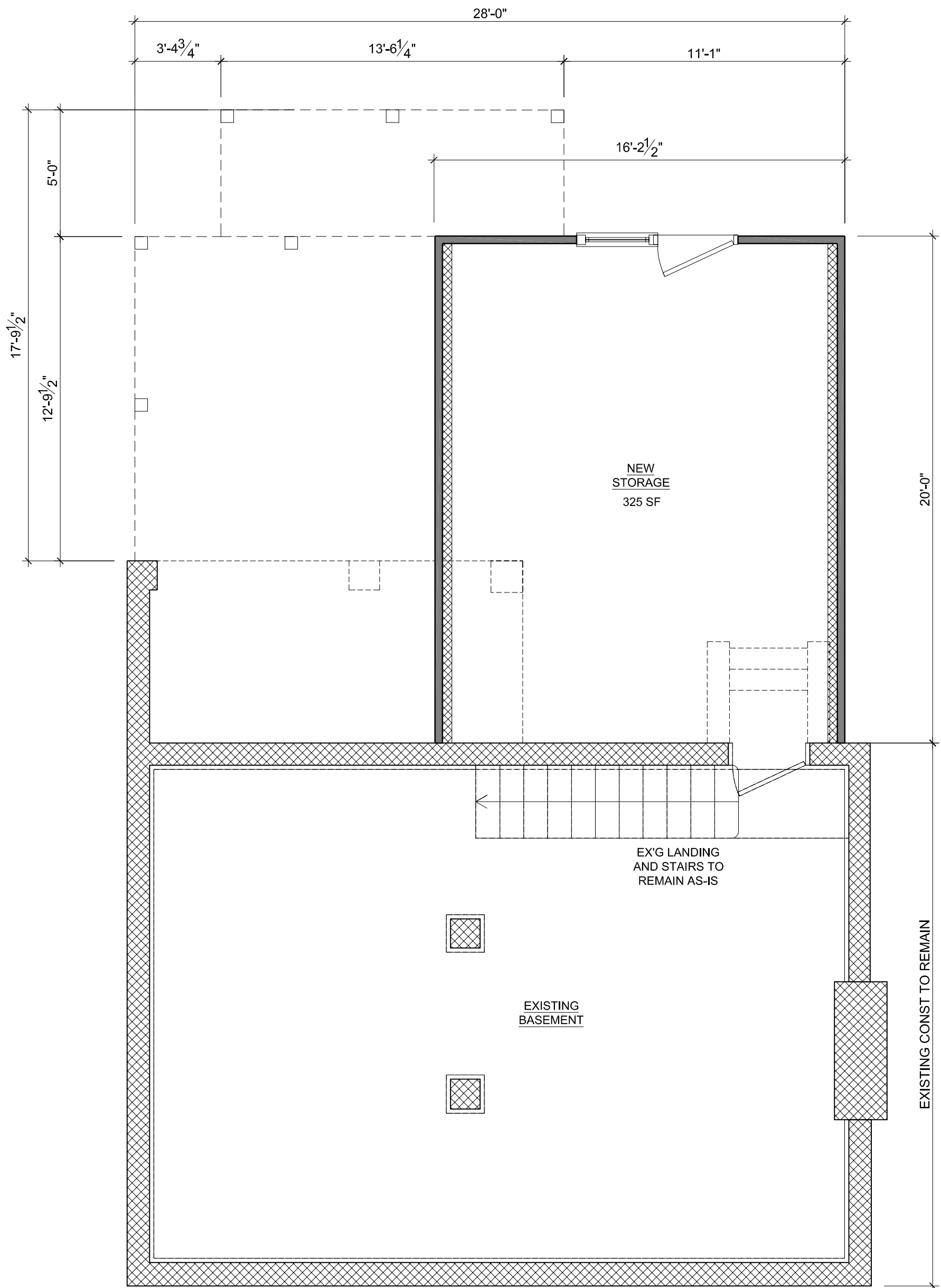
1 NEW BASEMENT FLOOR PLAN W/ DEMO 1/4" = 1'-0"
