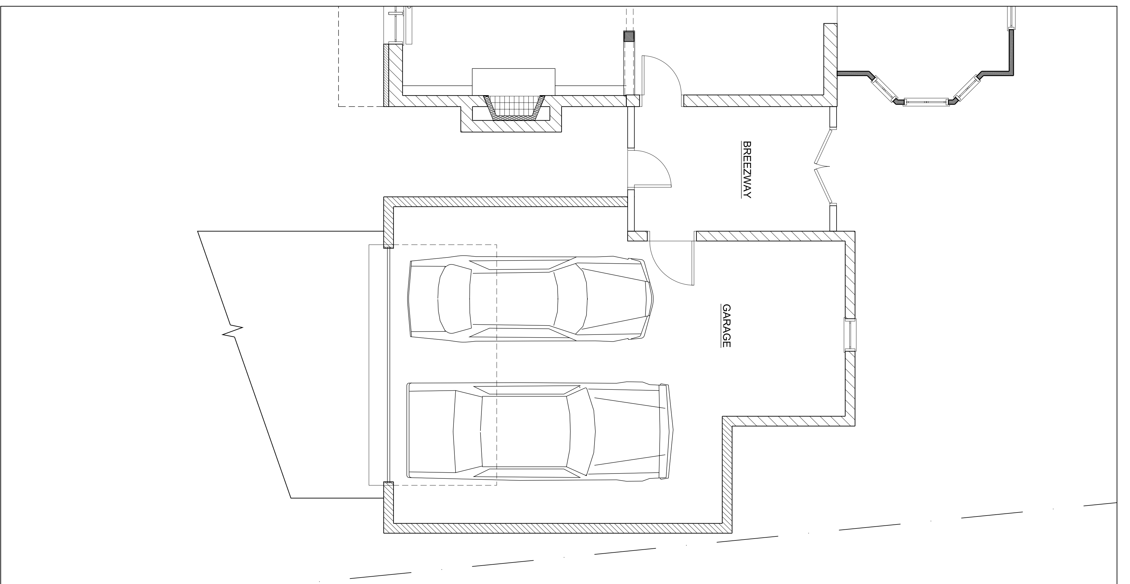
1 GARAGE "C" 1/4" = 1'-0"
