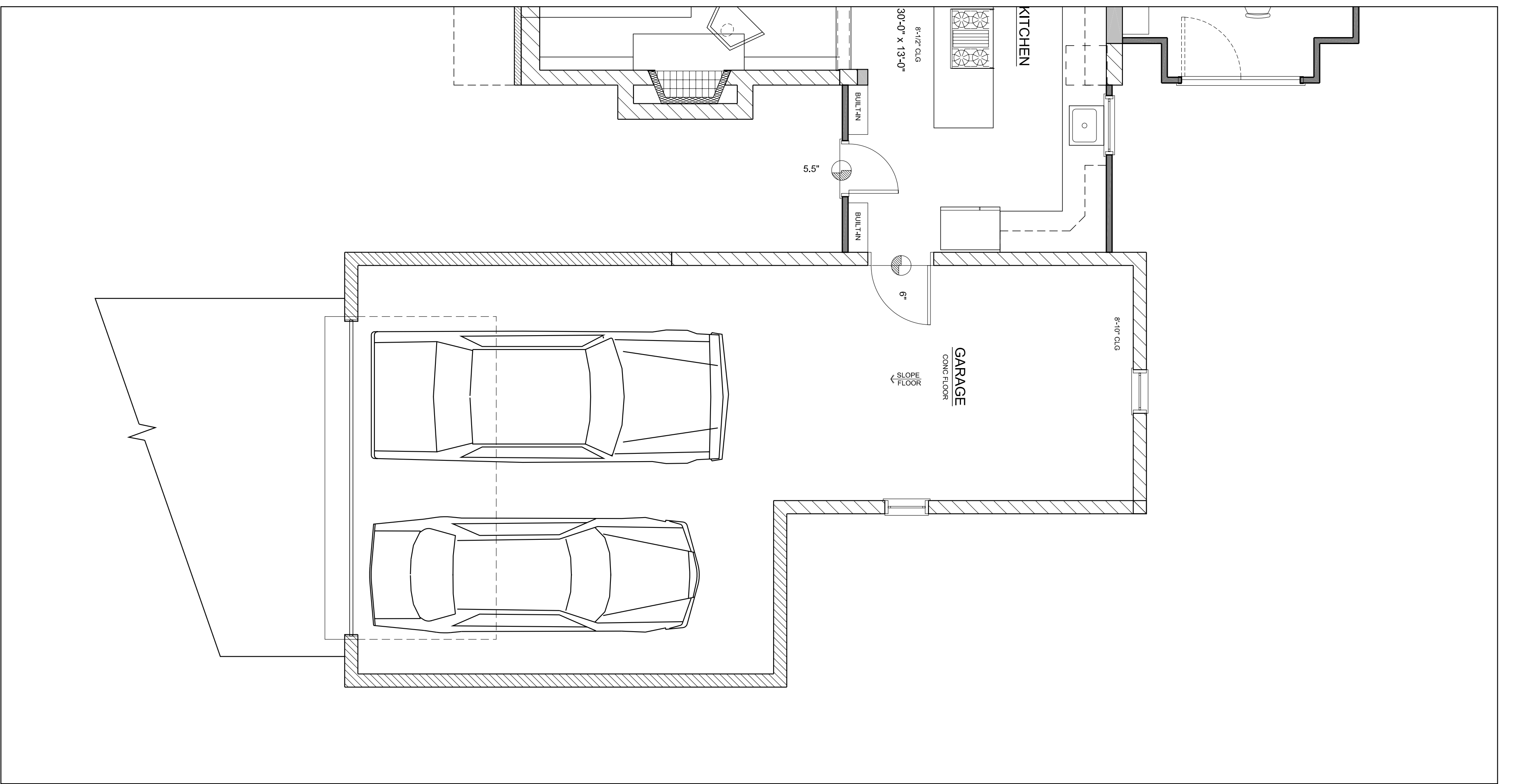
1 GARAGE "A" 1/4" = 1'-0"
