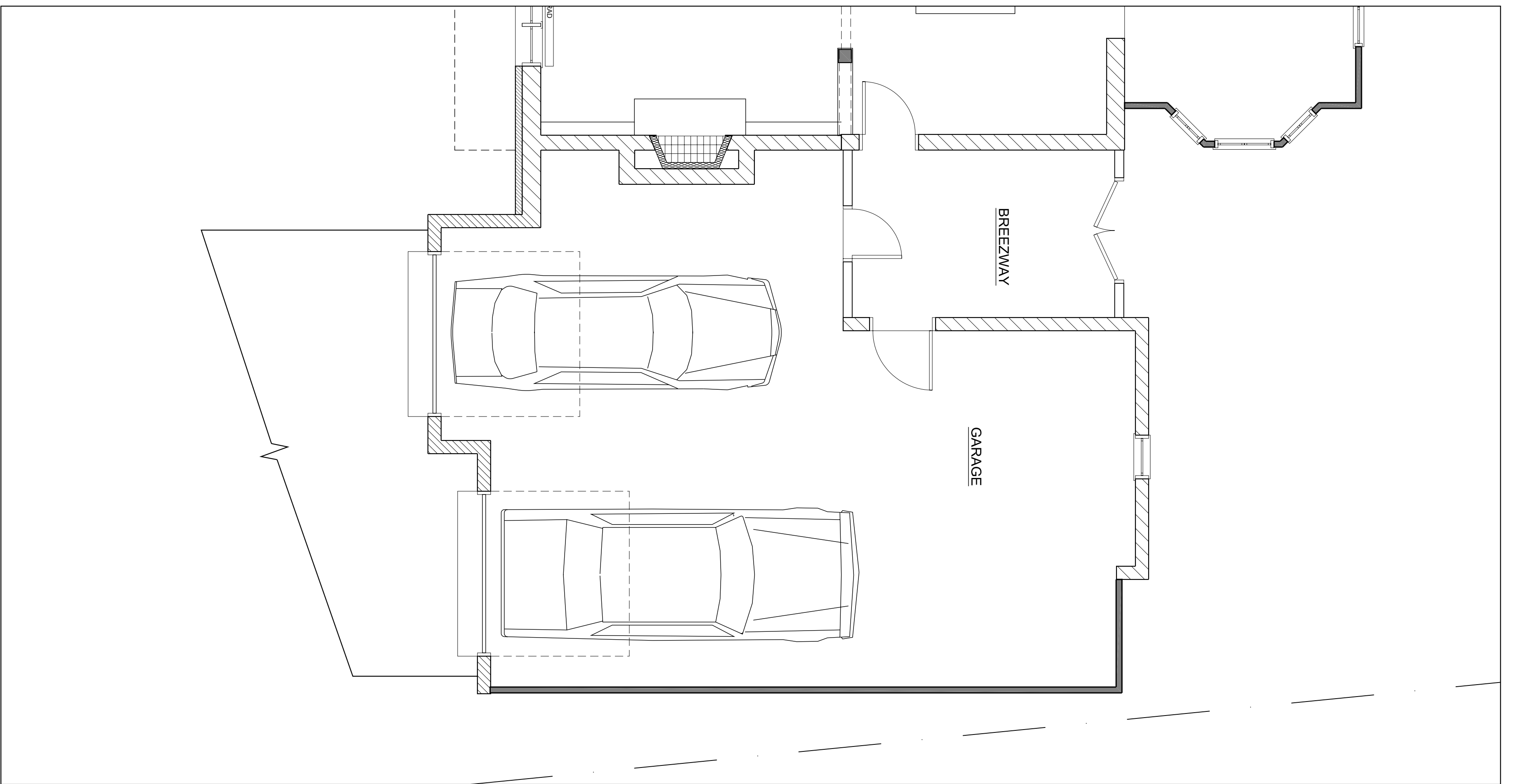
1 GARAGE "B" 1/4" = 1'-0"
